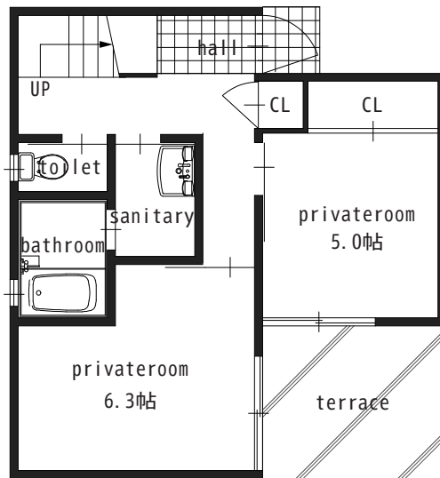
1F PLAN
